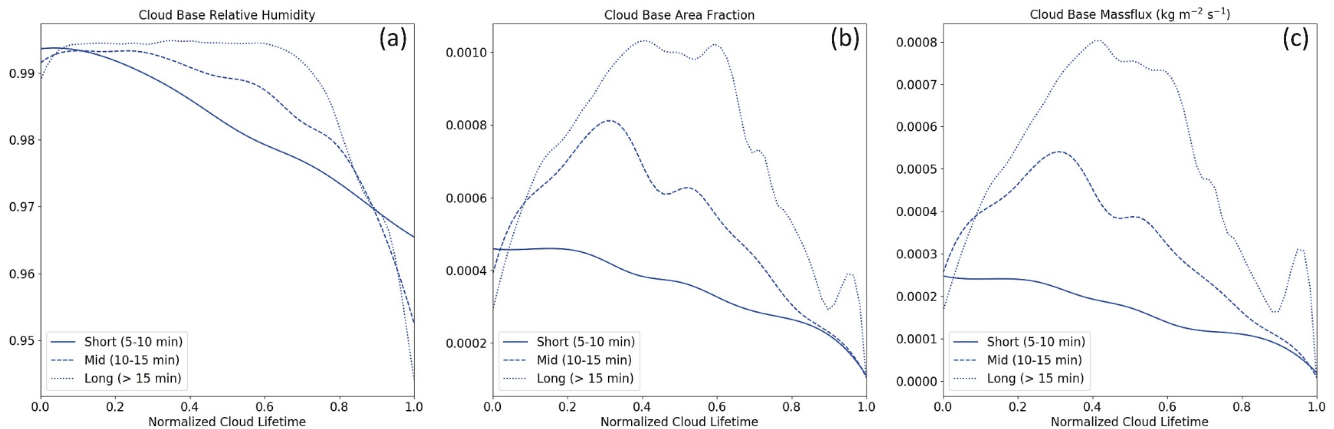
Figure 5. Evolution of (a) cloud base relative humidity, (b) cloud base area fraction and (c) cloud base mass-flux ( \text{kg m}^{-2} \text{s}^{-1} ), with normalized cloud lifetime. The solid, dashed and dotted lines represent the same groups of clouds that have sub-cloud coherent updrafts attached at each normalized lifetime as in Figure 4.
